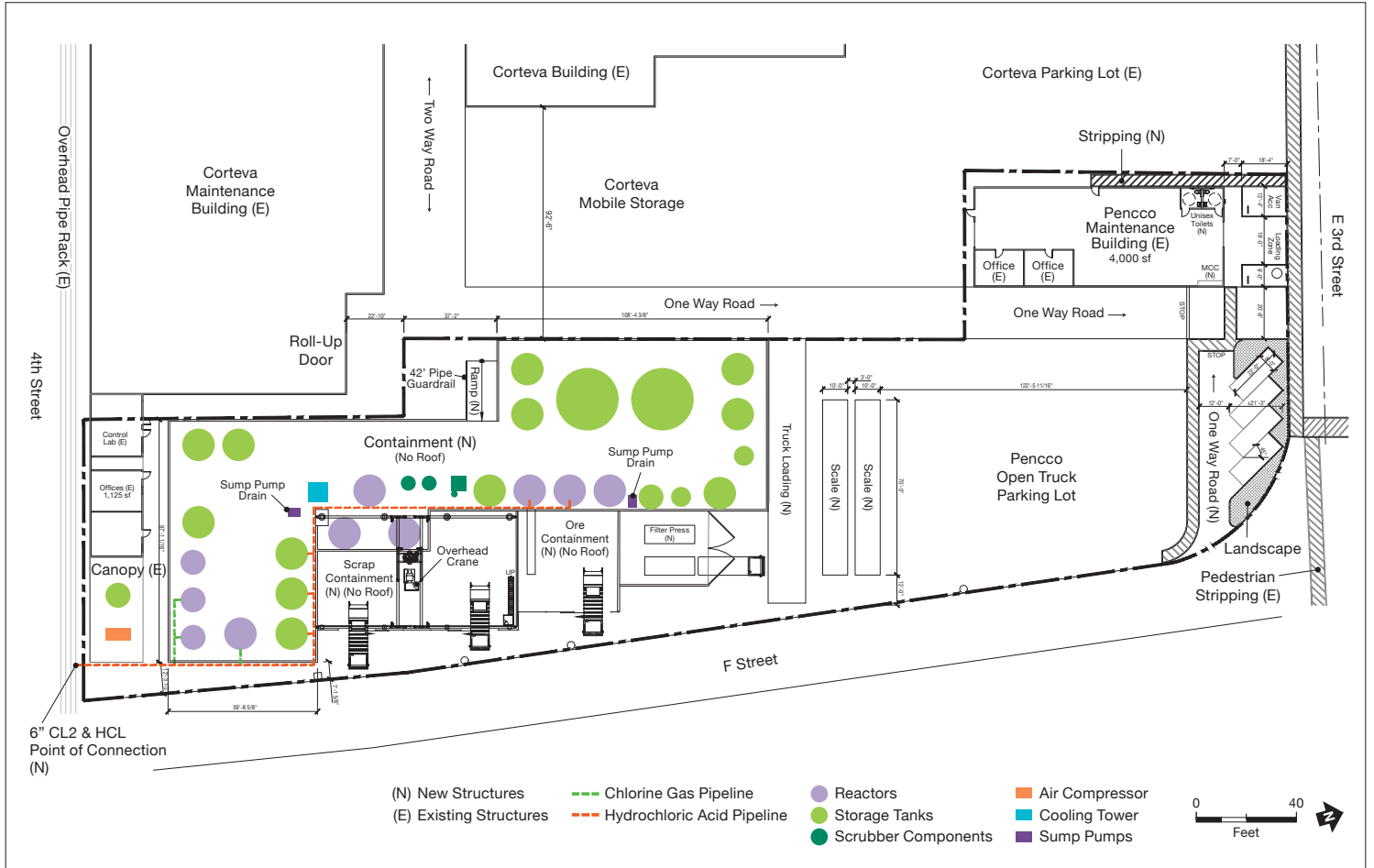
Figure 3 Site Plan
